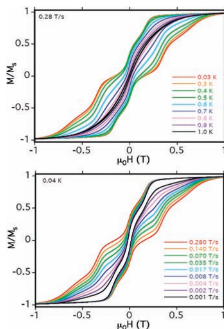
Figure 6. Hysteresis loops in plots of magnetization vs dc field for a single crystal of 3 \cdot xCH_2Cl_2 (top) at the indicated temperatures at 0.28 T/s and (bottom) at the indicated field scan rates at 0.04 K. M is normalized to its saturation value, M_s .
